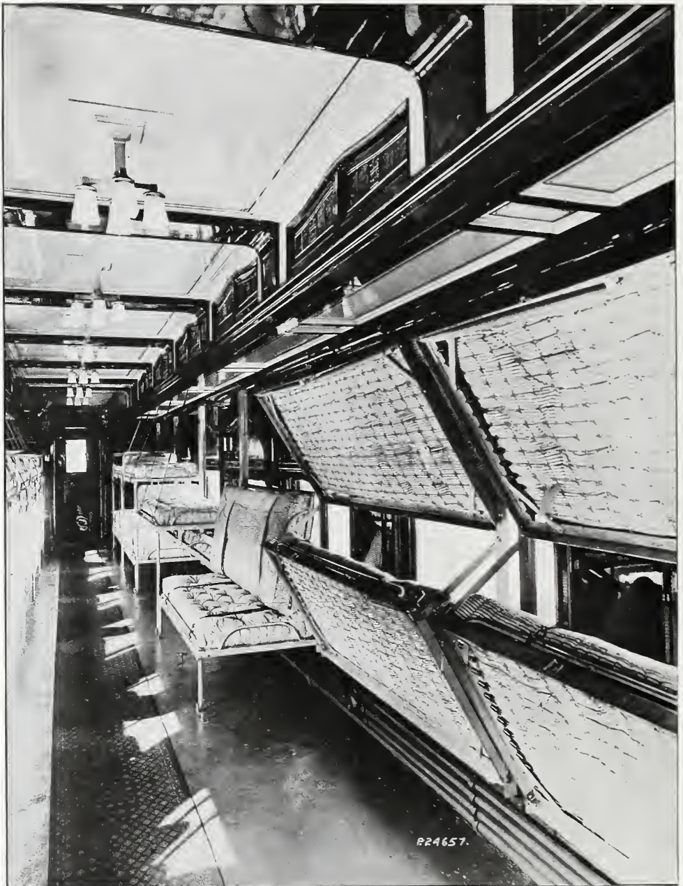
FIG. 78.—Hospital unit car fitted with Glennan adjustable bunks, showing manner of adjustment.
